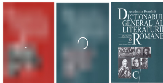
Figure 6. Image Loader
