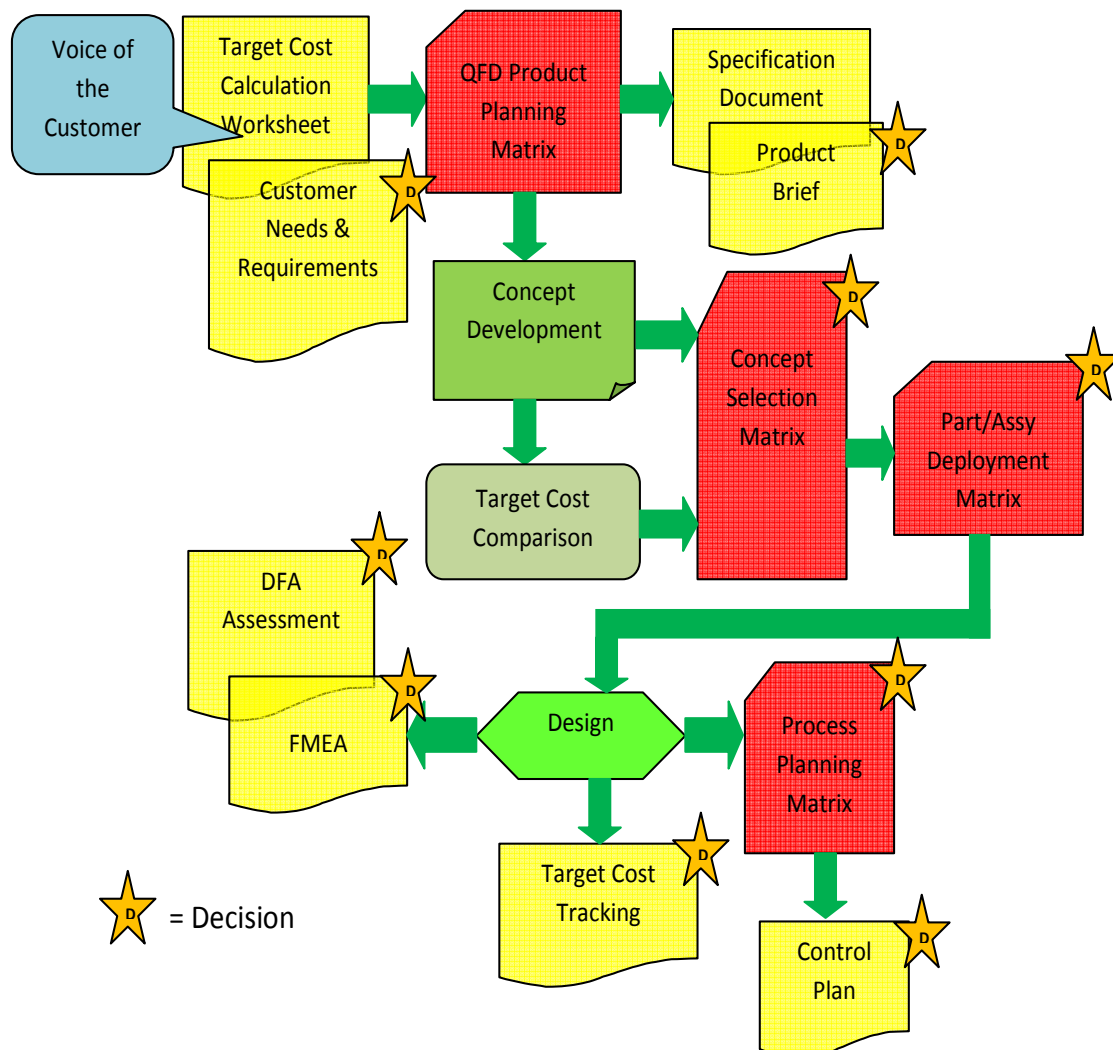
Figure 1. Planning and advanced design process of the product and processes with decision fields
