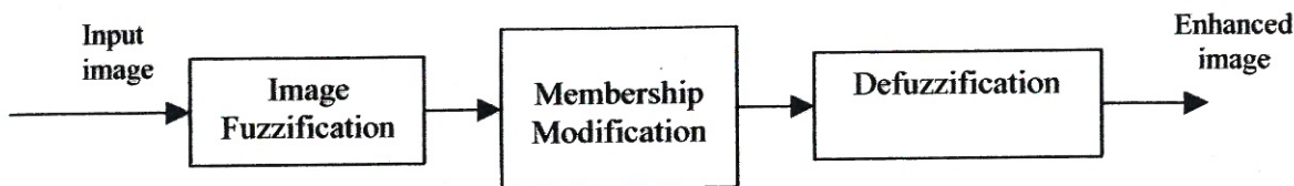
Figure 1: The Main Principles of Fuzzy Image Enhancement
