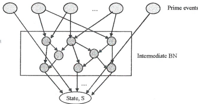
Figure 2: BN Model
